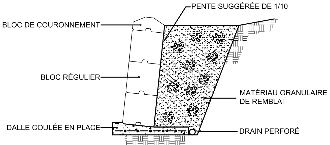
COUPE "A - A"
